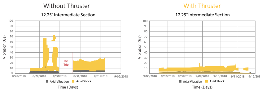
Axial Shock and Vibration Comparison
